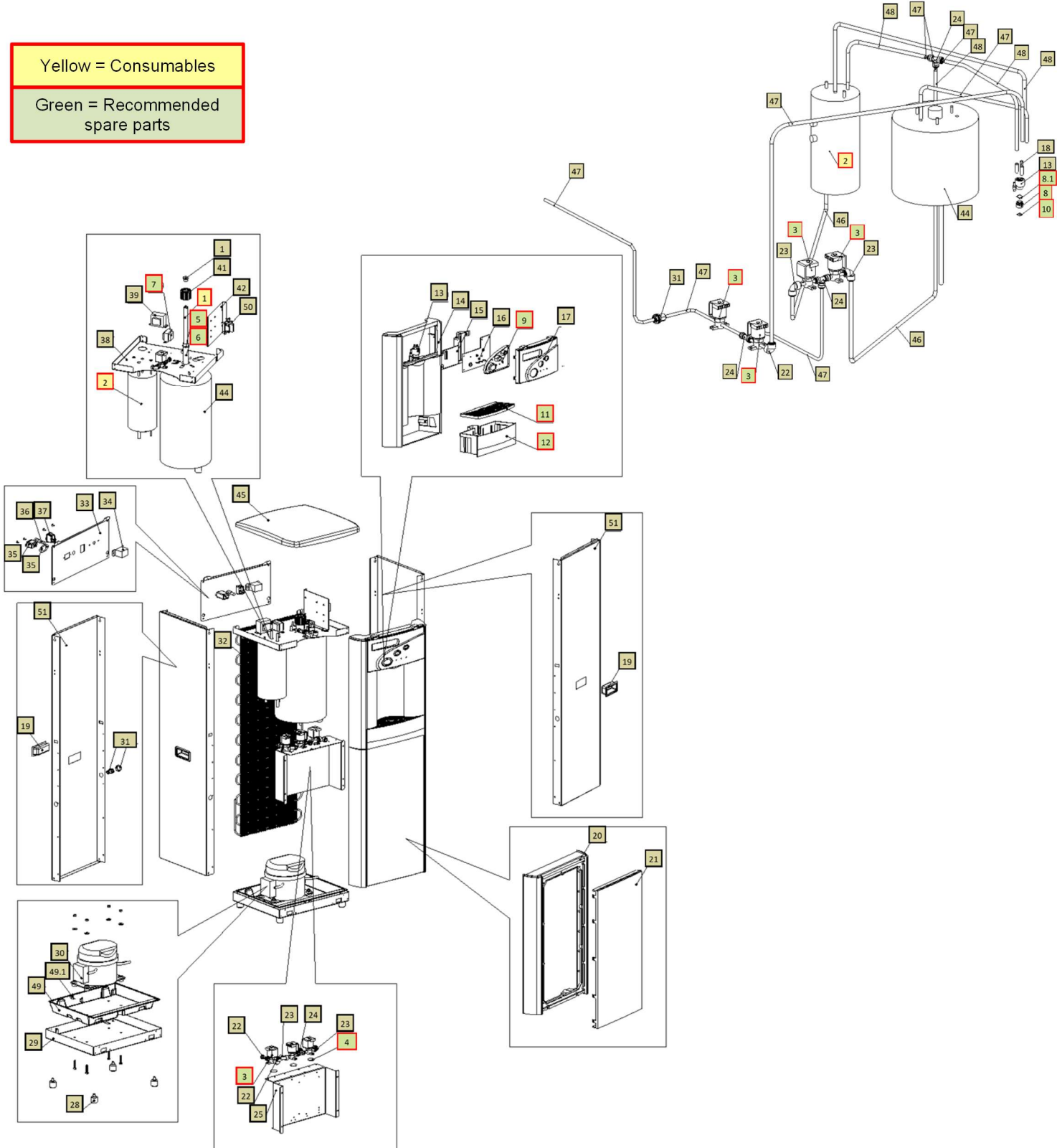
Wetted Drawing
