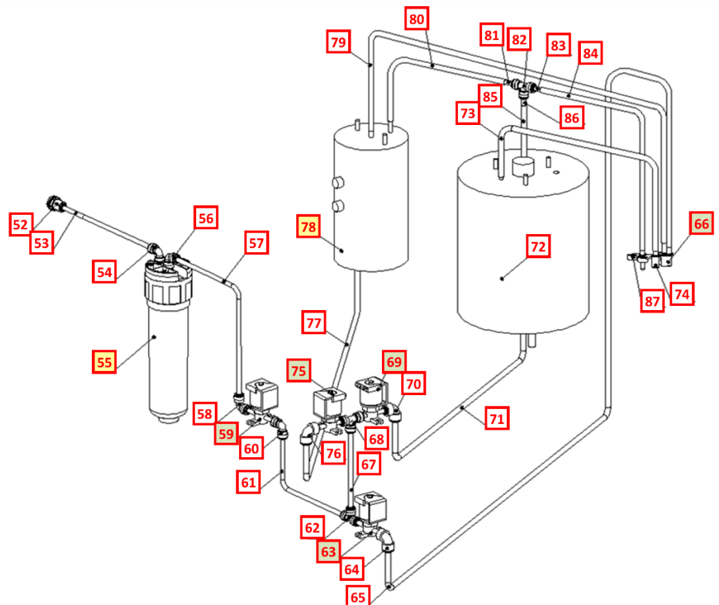
Wetted Drawing
